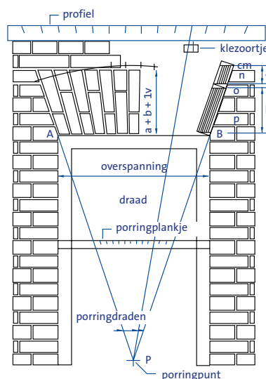
[Fig 22] Strek of hanekam
